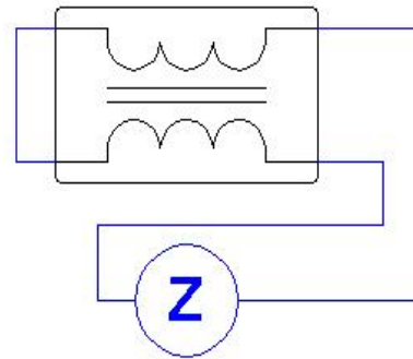
(B):Differential mode
